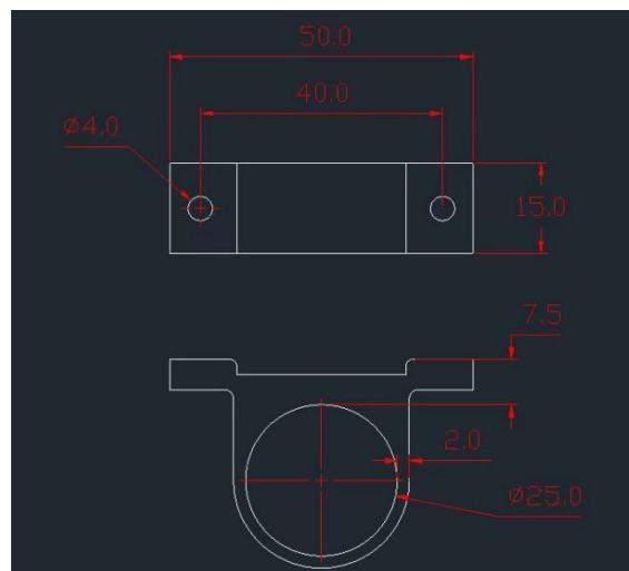
Dimensional Outline Drawing (Unit:mm)
